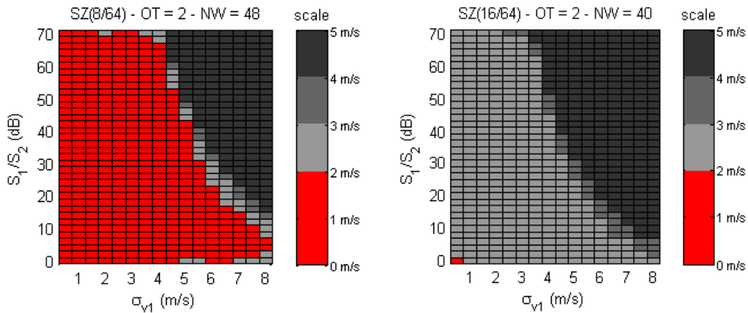
Fig. 4.8. Examples of good (left panel) and bad (right panel) phase code-PNF width combinations in terms of weak-trip recovery.
