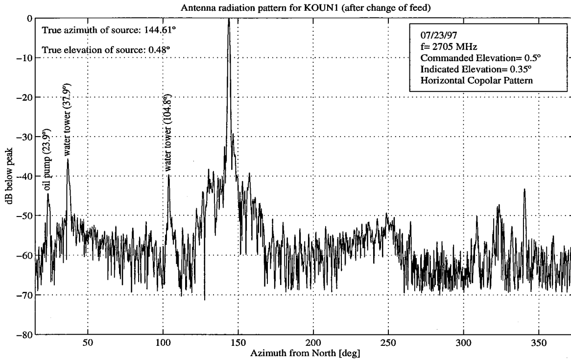
Fig. II.8 (a) The 0° cut pattern through the boresight (commanded elevation angle is 0.5°) for a scan of KOUN1 copolar H radiation after the dual-port feed was installed. (The beam axis is at a commanded elevation angle of 0.5°.) The front port is connected to the receiver.
